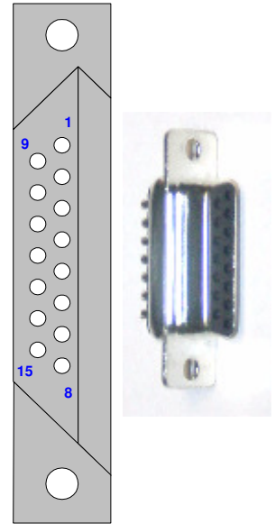
DB-15S (rear view)
